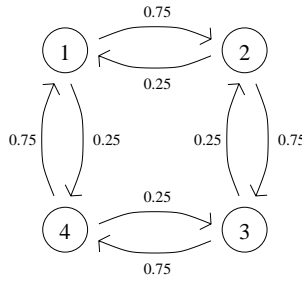
Fig. 6. Transition graph of the Markov chain in Example 6.3.
